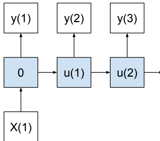
Figure 5.3: One-to-Many Sequence Prediction Model.
