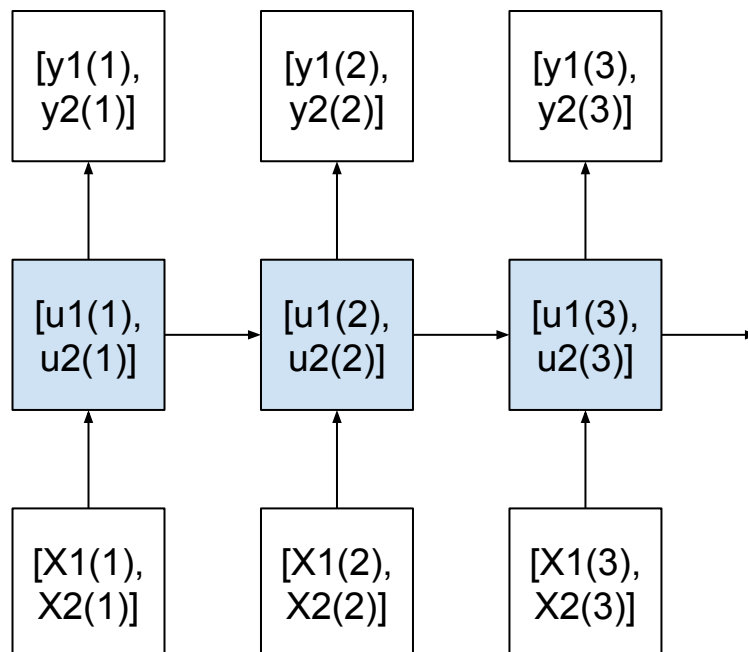
Figure 5.6: Multiple-Feature Sequence Prediction Model.
