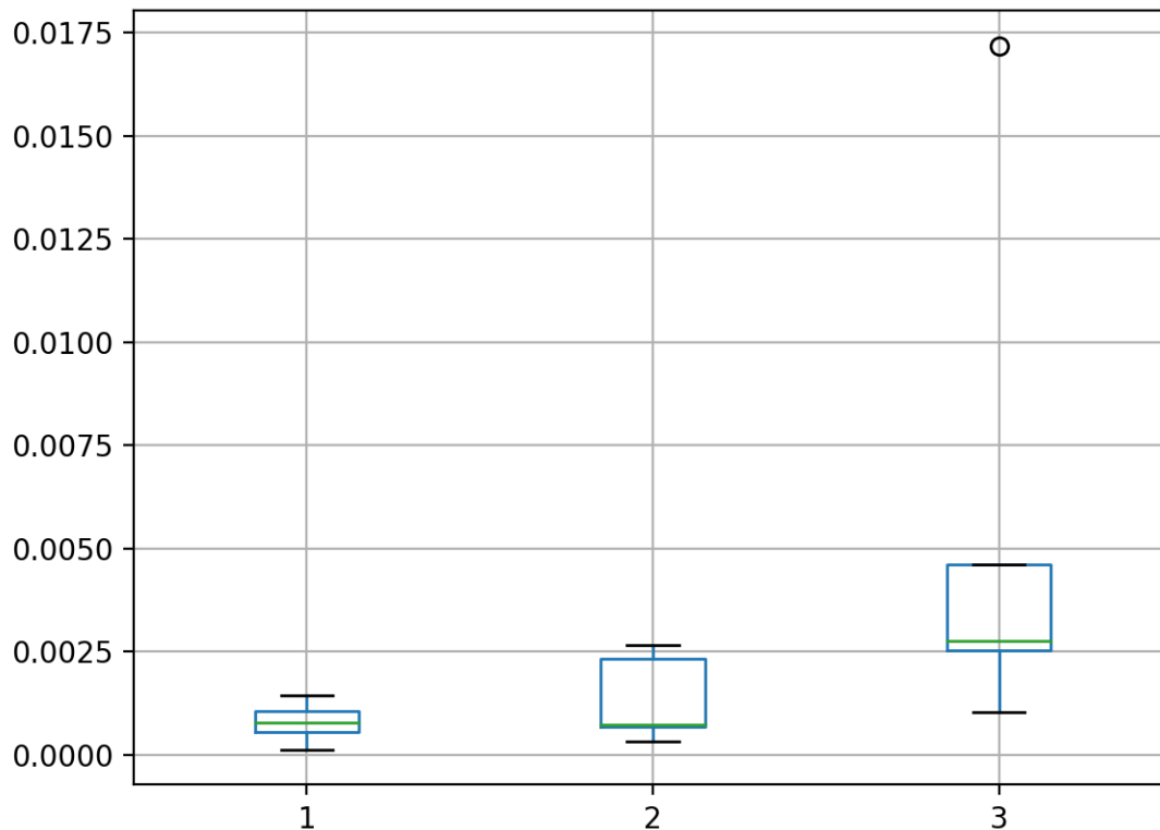
Figure 12.7: Box and whisker plots of the results of tuning the batch size.
