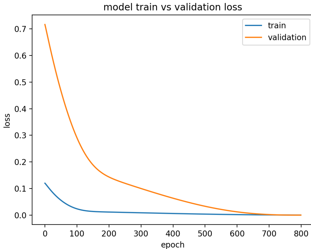
Figure 12.3: Diagnostic line plot of well fit model.
