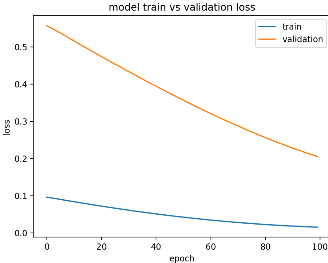
Figure 12.1: Diagnostic line plot of underfit model with more training to do.
