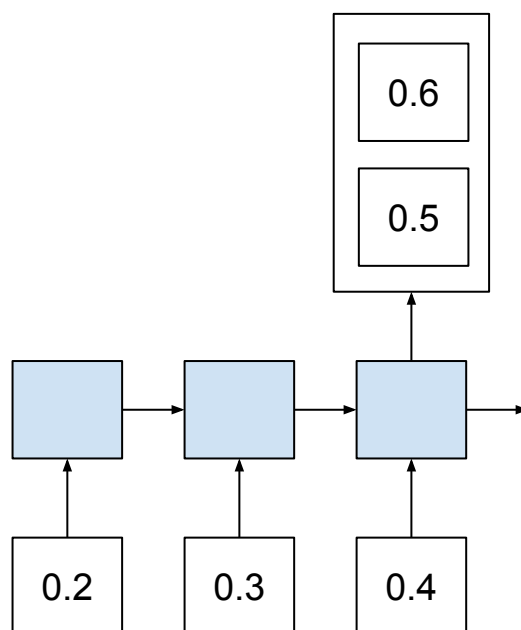
Figure 7.5: Damped sign wave prediction problem framed with a many-to-one prediction model.
