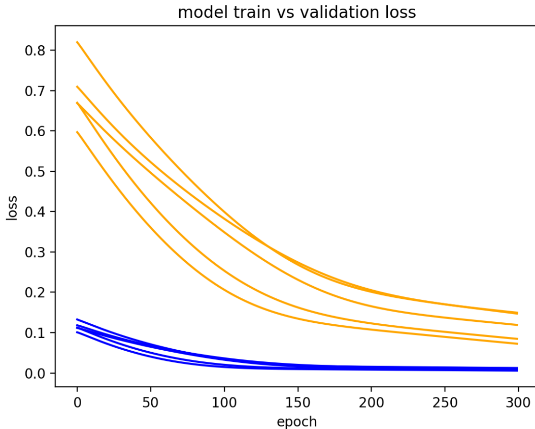
Figure 12.5: Diagnostic line plot of multiple model runs.
