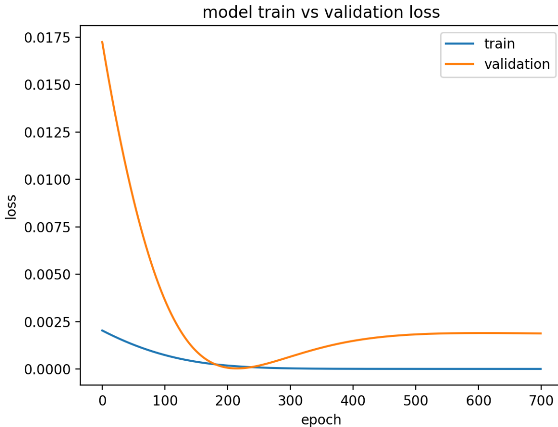
Figure 12.4: Diagnostic line plot of an overfit model.
