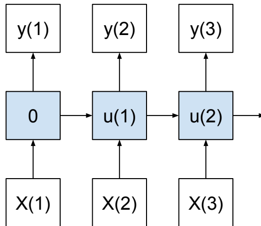
Figure 5.2: One-to-One Sequence Prediction Model Over Time.
