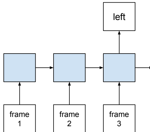
Figure 8.2: Moving square video prediction problem framed with a many-to-one prediction model.
