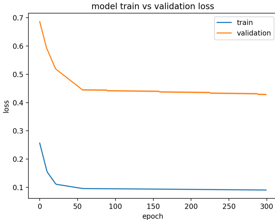
Figure 12.2: Diagnostic line plot of underfit model where are larger model may be needed.
