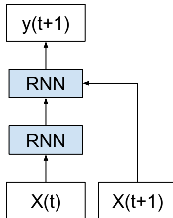
Figure 2.3: Example of an unfolded recurrent neural network with layers.
