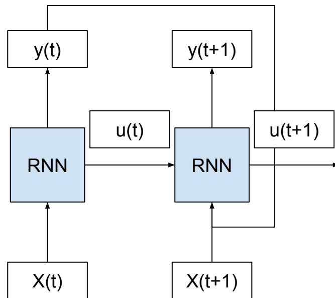
Figure 2.2: Example of an unfolded recurrent neural network.
