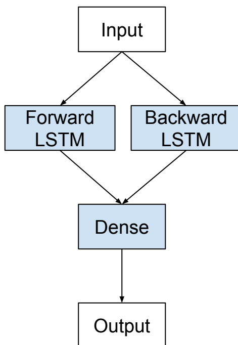
Figure 10.1: Bidirectional LSTM Architecture.
