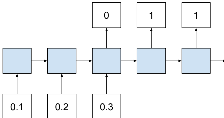
Figure 10.2: Cumulative sum prediction problem framed with a many-to-many prediction model.
