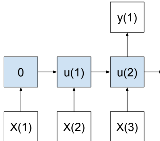
Figure 5.4: Many-to-One Sequence Prediction Model.
