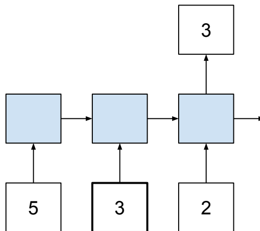
Figure 6.2: Echo sequence prediction problem framed with a many-to-one prediction model.
