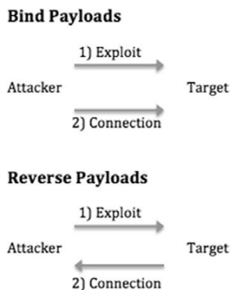
FIGURE 4.7 Difference between Bind and Reverse Payloads.
